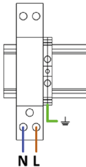
Figure 6-4 - Parafoudre
