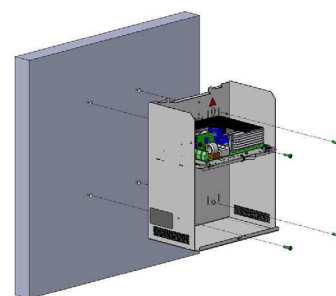
C38 – Dim : 289x350x189mm – IP31
