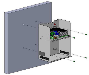
C38 – Dim : 289x350x189mm – IP31
