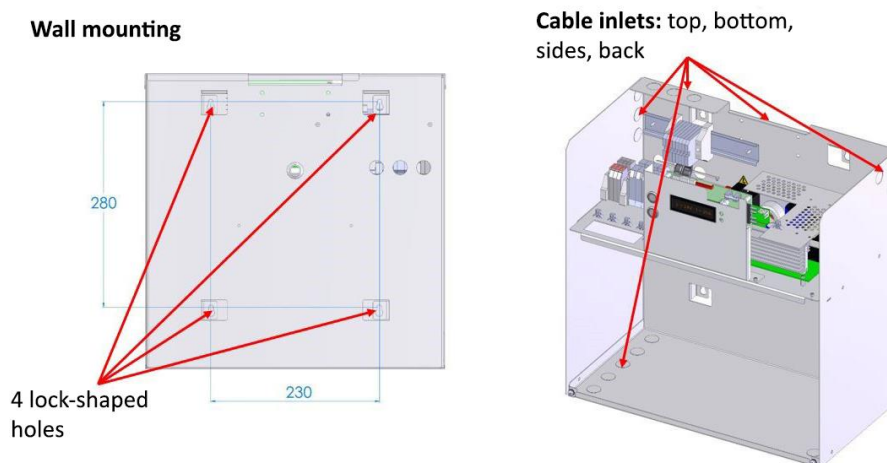
Figure 2: Wall-mounting and cable inputs
