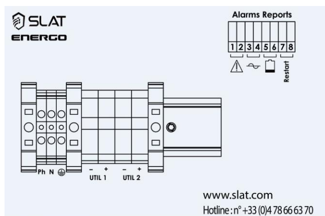
Figure 3: ENERGO model connection terminals, 2 fused user feeders
