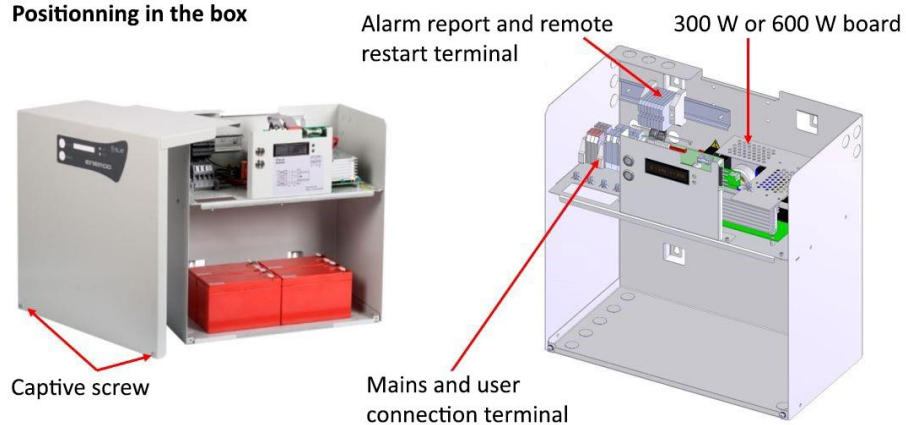
Figure 1: Location of component parts
